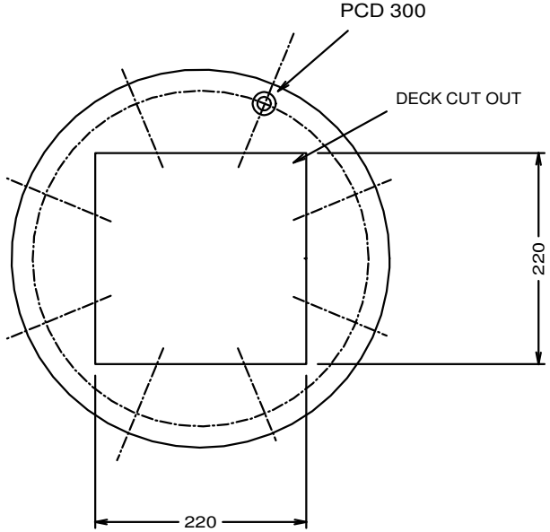
MOUNTING DETAIL
